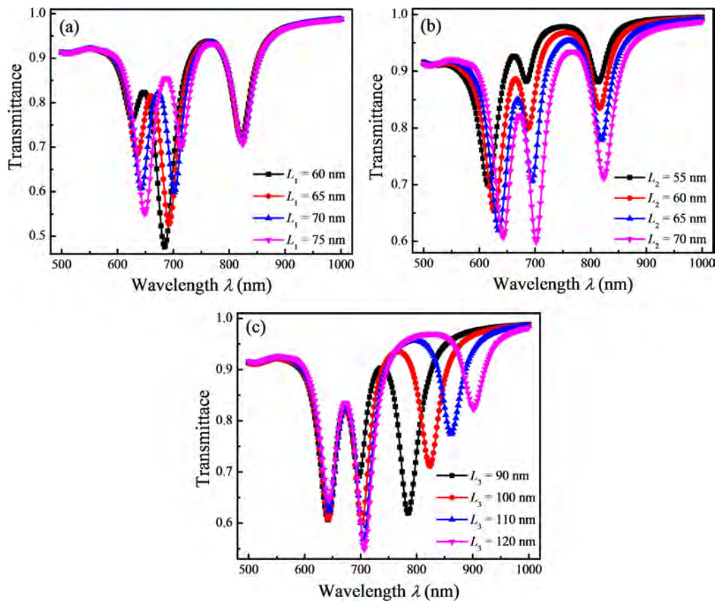
Fig. 4. Transmittance spectra of the PDS with different nanorod lengths: (a) different L_1 ; (b) different L_2 ; (c) different L_3 .
