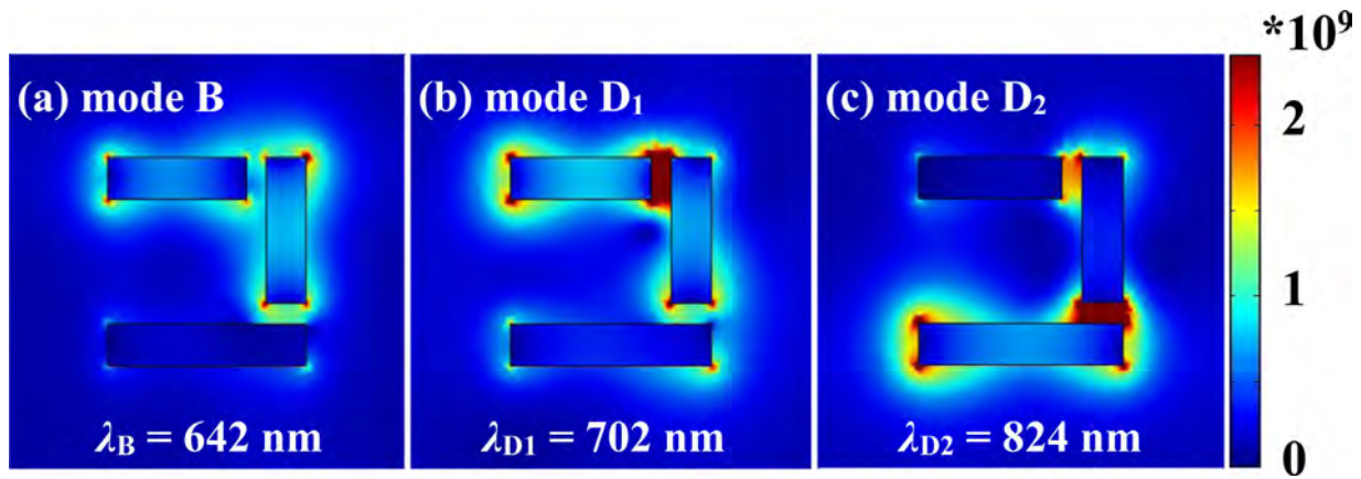
Fig. 3. Electric field distributions of the PDS at different modes (a) mode B, (b) mode D 1 , and (c) mode D 2 .
