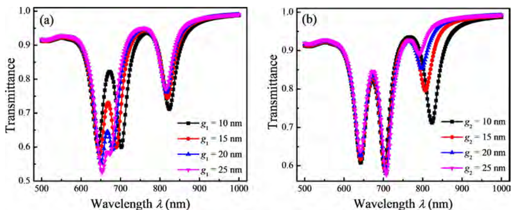
Fig. 5. Transmittance spectra of the PDS with different gaps: (a) different g_1 ; (b) different g_2 .
